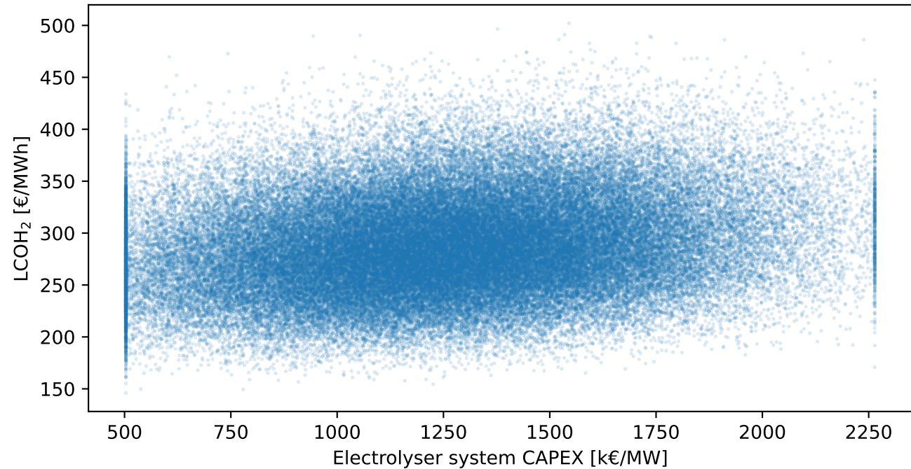
LCOH 2 vs Electrolyser CAPEX
